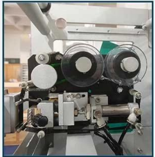
Date printer
