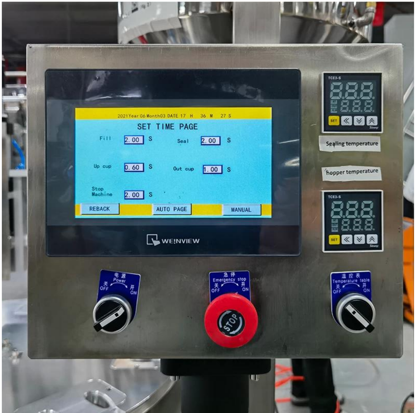
Touch-Screen
