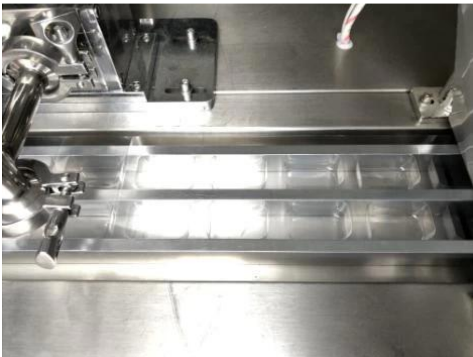
shaping device
