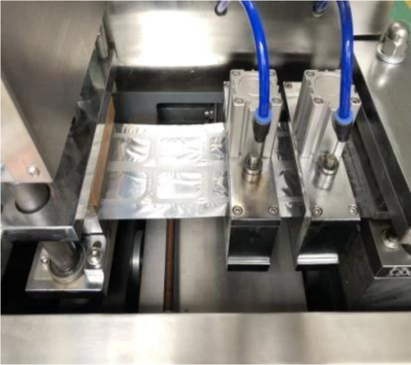
sealing device
