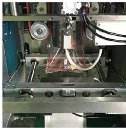
Bag Cutter Device
