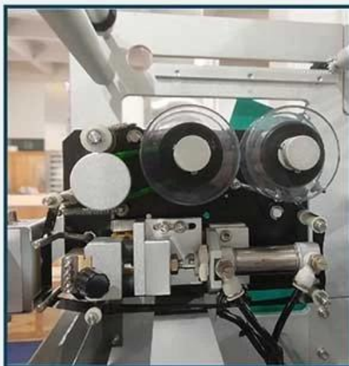
Date printer
