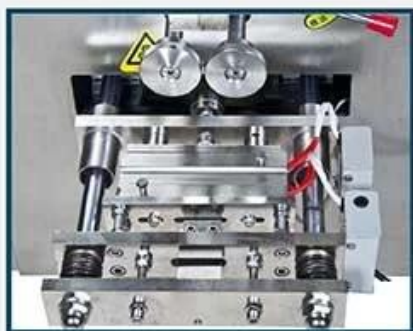
Transverse sealing structure
