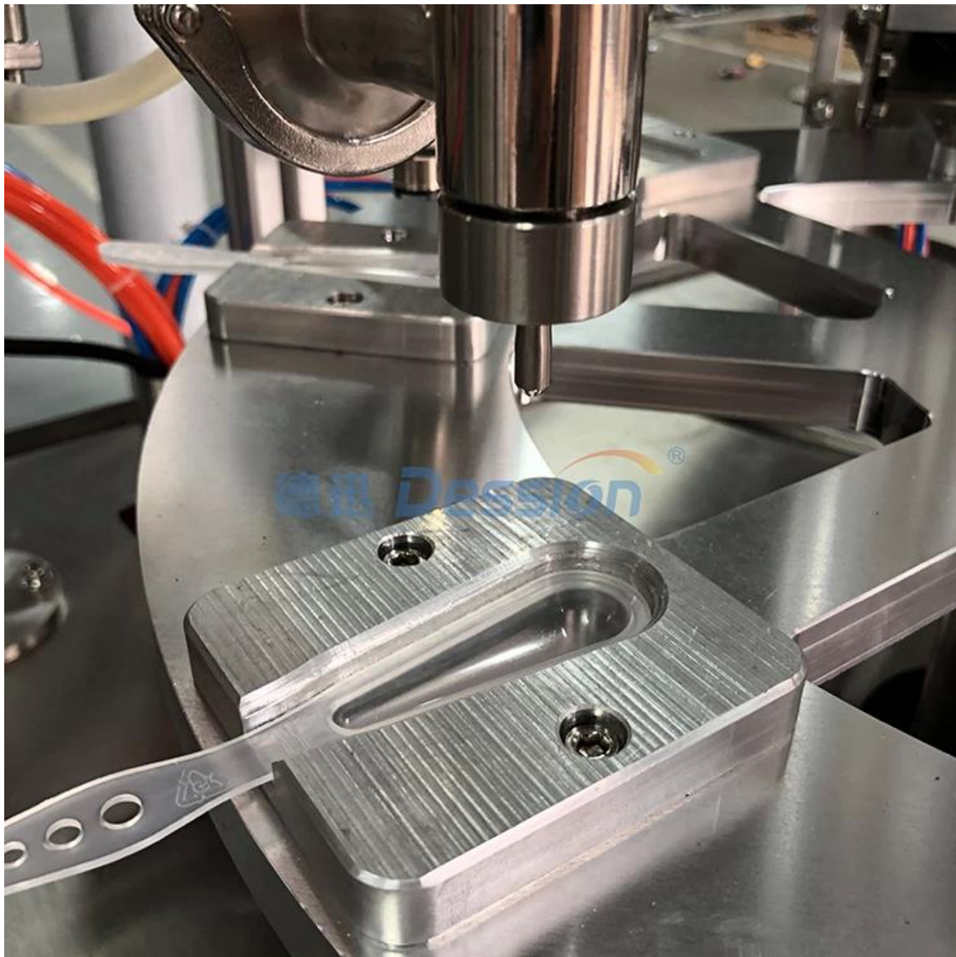
Filling device
