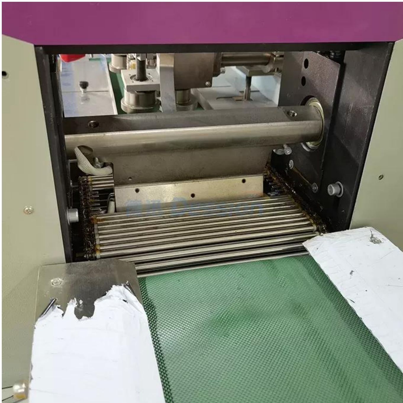
Cutting Device
