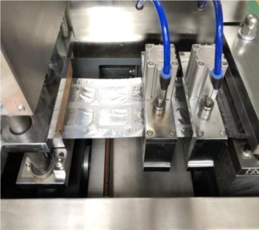
sealing device
