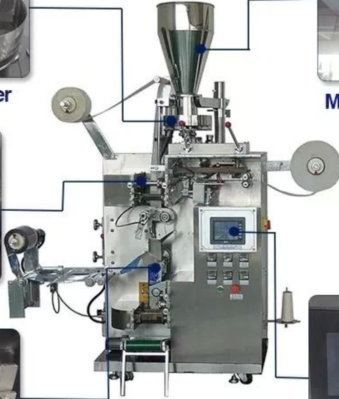
Outer bag sealing device
