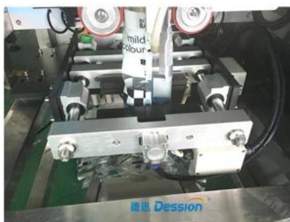
Cutting Knife
